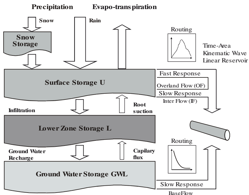
Figure 2.1 Model structure for the RDI model.
