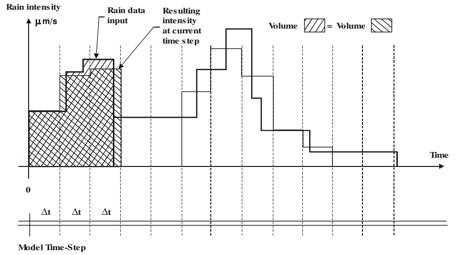
Figure 6.3 Rain Input Data vs. Model-applied data
