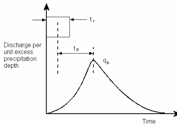
Figure 5.2 Snyder's Synthetic Unit Hydrograph
