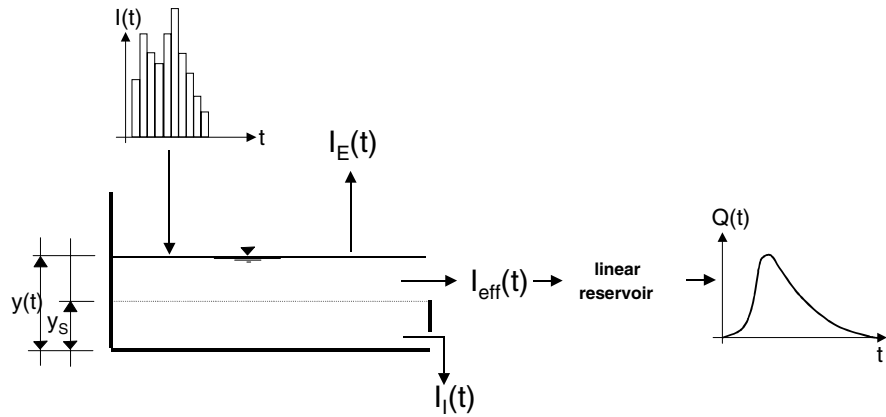
Figure 4.4.1 The processes simulated in the surface runoff model C.
