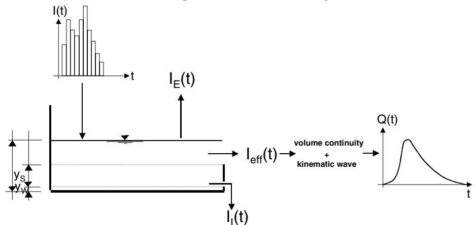
Figure 3.3.1 The simulated processes in the Surface runoff model B.
