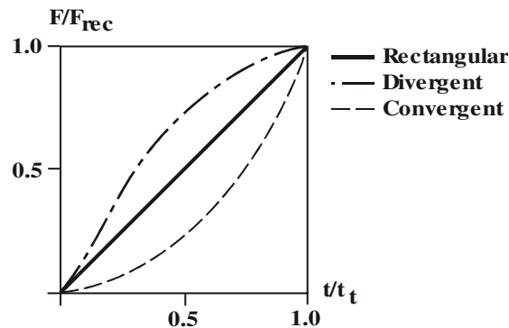
Figure 2.1 The three pre-defined time/area curves available in MOUSE
