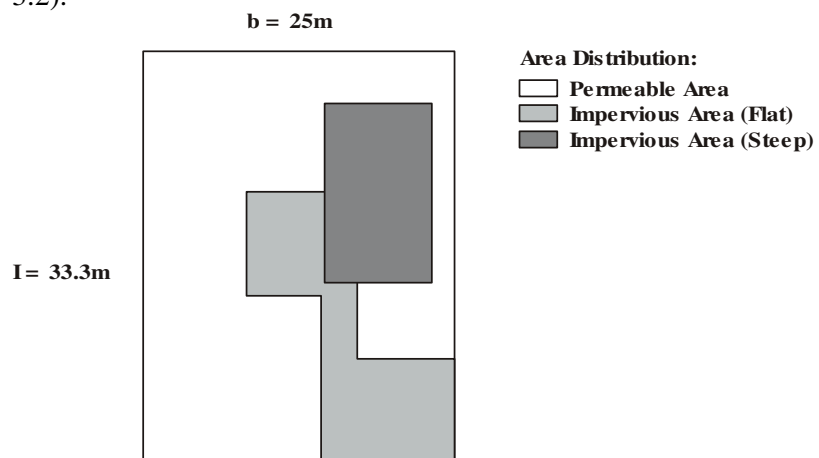
Figure 3.3.2 Sub-catchments with total area = 833 m 2 .
